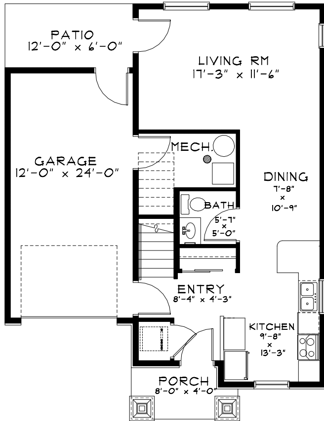
FIRST FLOOR PLAN 2 BEDROOM UNIT 632 S.F.
