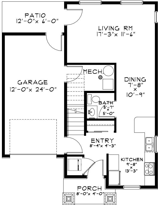
FIRST FLOOR PLAN 3 BEDROOM UNIT 632 S.F.
